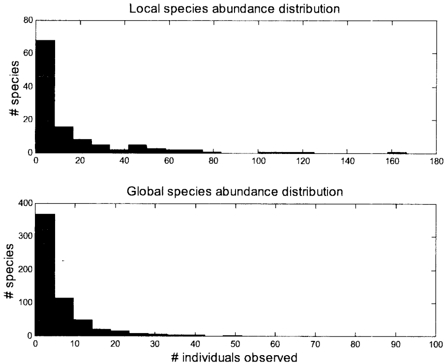
Fig. 1. The top graph is an empirically observed example of a local species abundance distribution (SAD) for the BBS route at 100.217°W longitude, 48.883°N latitude in North Dakota near the Canadian border. There are many species with a very low abundance (left side of graph). There are a few species with a high abundance (right side of graph). This shape is sometimes called a 'hollow curve'. The bottom graph gives a species abundance distribution for global abundance. In this case, global abundance is measured by abundance averaged across the range (AVGABUND), but the pattern is similar for other measures of global abundance. Note that the global SAD also is distributed with a hollow curve, just as local SADs are. Our model predicts that these two curves should have the same shape (although not the same scale). We examine quantitative evidence for this similarity in the text.
