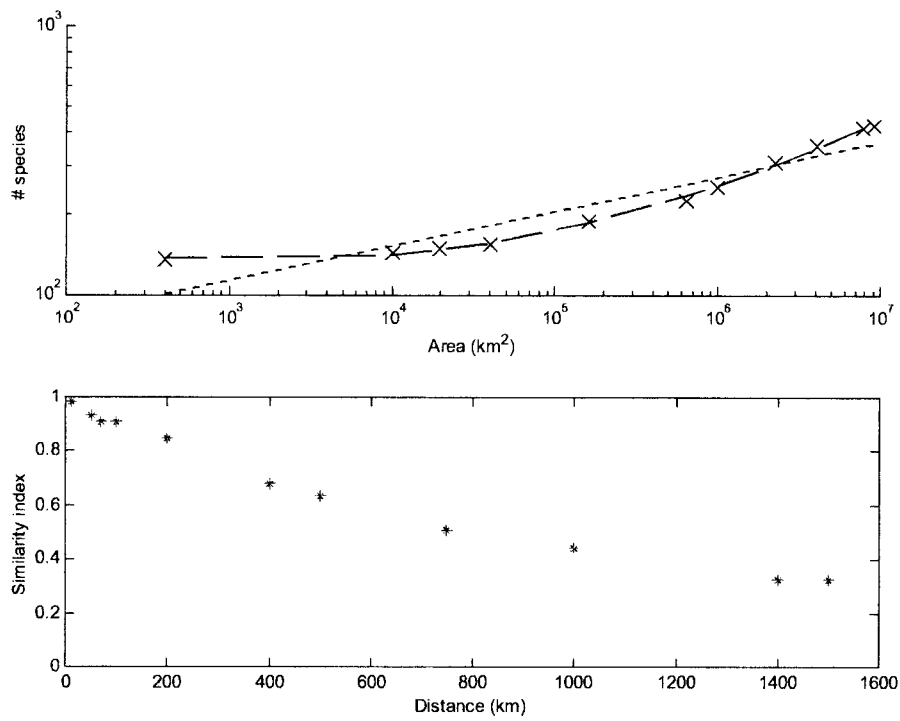
Fig. 4. The top figure shows a classic species–area relationship (SPAR) with log area (in \text{km}^2 ) on the x-axis and log number of species on the y-axis. The \times symbols represent the simulation based on the theory in this paper with parameters as specified in Appendix 1 and the resampling method used. The dotted line is a straight-line (power law) fit to the simulation, whereas the dashed line is a quadratic fit to the simulation. The bottom plot shows a similarity–decay relationship. The y-axis plots similarity of species composition between an arbitrary starting point and various other points along a transect from the starting point. In this plot, community similarity is calculated using the Jaccard index. The x-axis plots linear distance in kilometres between the arbitrary starting point (here the centre of the square in the simulation) and select other points along a transect from the starting point (here chosen to be points due east of the starting point at various distances).
